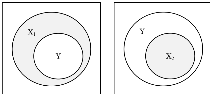
Figure 6.1 Necessary Condition and Sufficient Condition (Crisp Sets)
