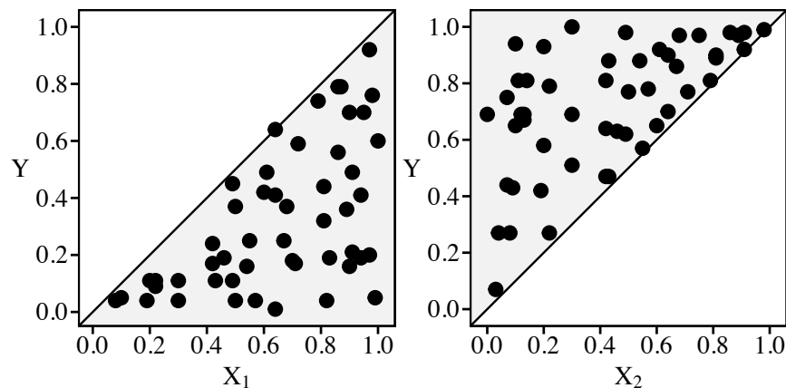
Figure 6.2 Necessary Condition and Sufficient Condition (Fuzzy Sets)
