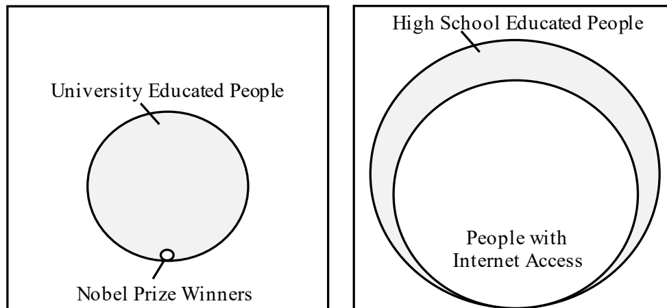
Figure 6.7 Two Types of Trivial Necessary Conditions
