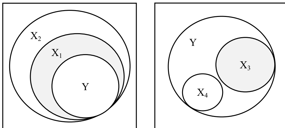
Figure 6.4 Coverage in Necessary and Sufficient Conditions (Crisp Sets)
