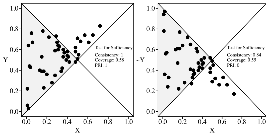
Figure 6.6 Simultaneous Subset Relations
