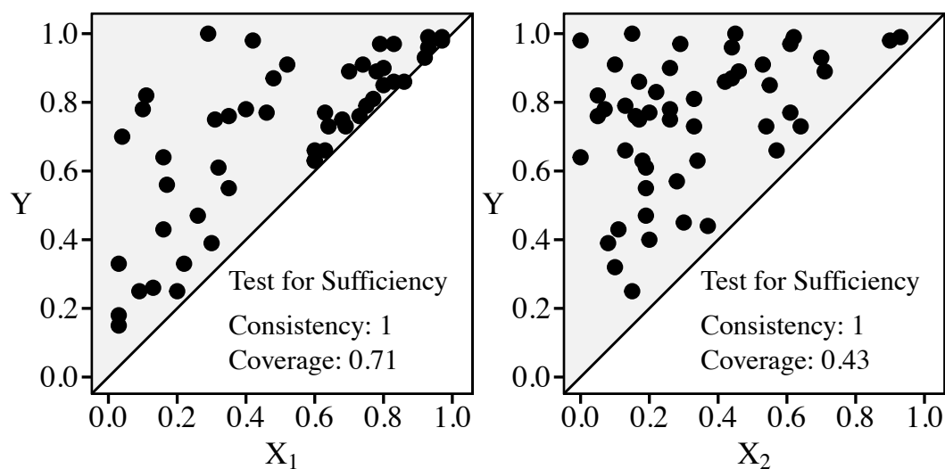
Figure 6.5 Sufficient Conditions with Varying Coverage (Fuzzy Sets)
