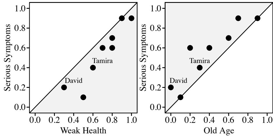
Figure 6.3 XY Plots: Risk Factors and Serious Symptoms
