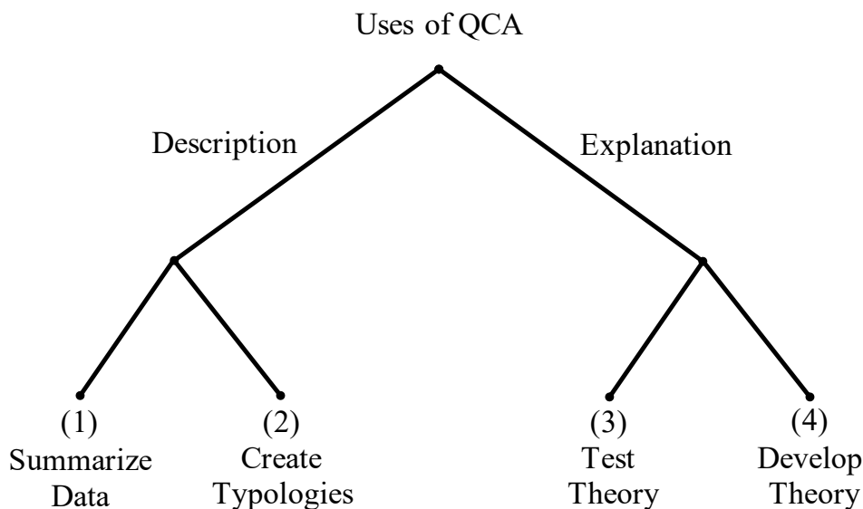
Figure 2.2 The Four Uses of QCA
